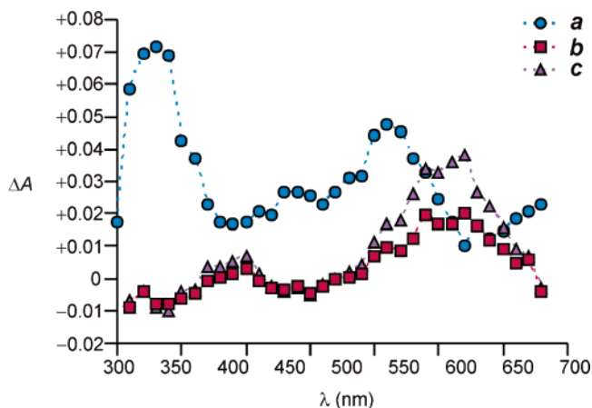
FIGURE 11. Absorption spectra recorded 0.2 \mu\text{s} after laser excitation (266 nm, \sim 8 mJ) of a degassed solution (0.03 mM, MeCN, 20 ^{\circ}\text{C} ) of 22 (a) and optically matched solutions of SP6 (b) and SP7 (c).
