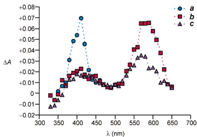
FIGURE 8. Absorption spectra recorded 0.2 \mu s after laser excitation (266 nm, ~8 mJ) of a degassed solution (0.03 mM, MeCN, 20 °C) of 20 (a) and optically matched solutions of SP1 (b) and SP3 (c).
